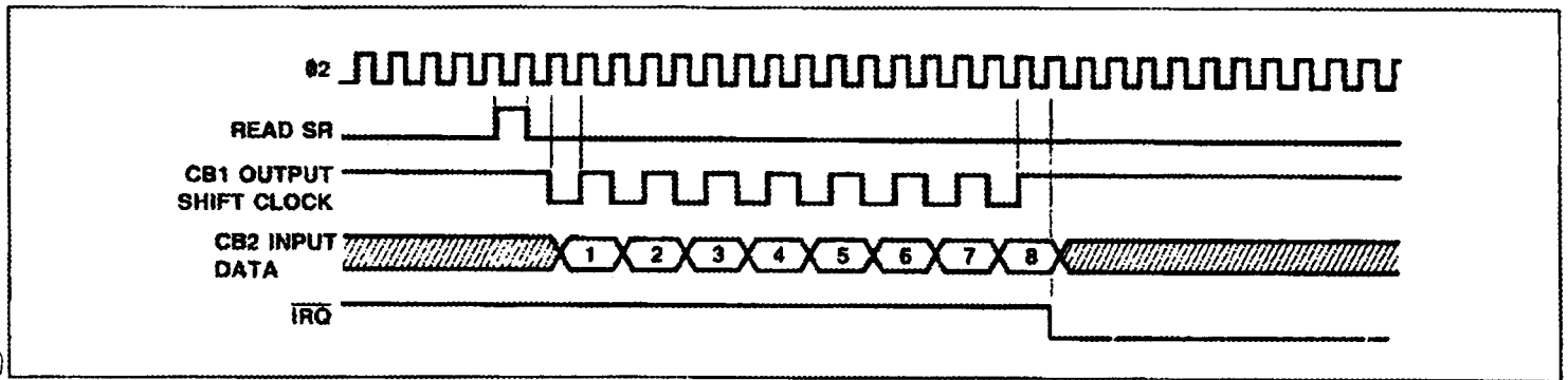
Figure 23. SR Mode 2 — Shift In Under #2 Control
