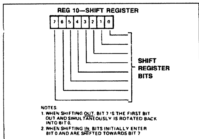
Figure 20. Shift Register
