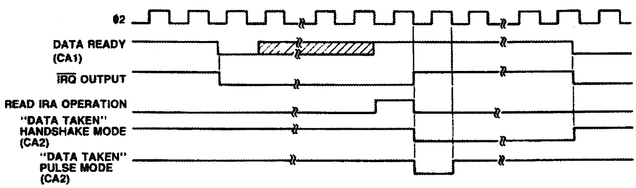
Figure 9. Read Handshake Timing (Port A Only)
