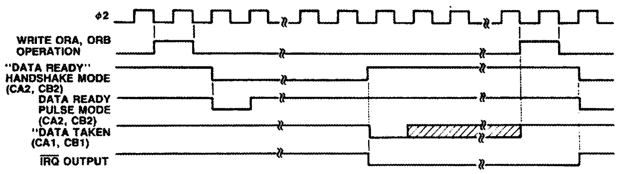
Figure 10. Write Handshake Timing
